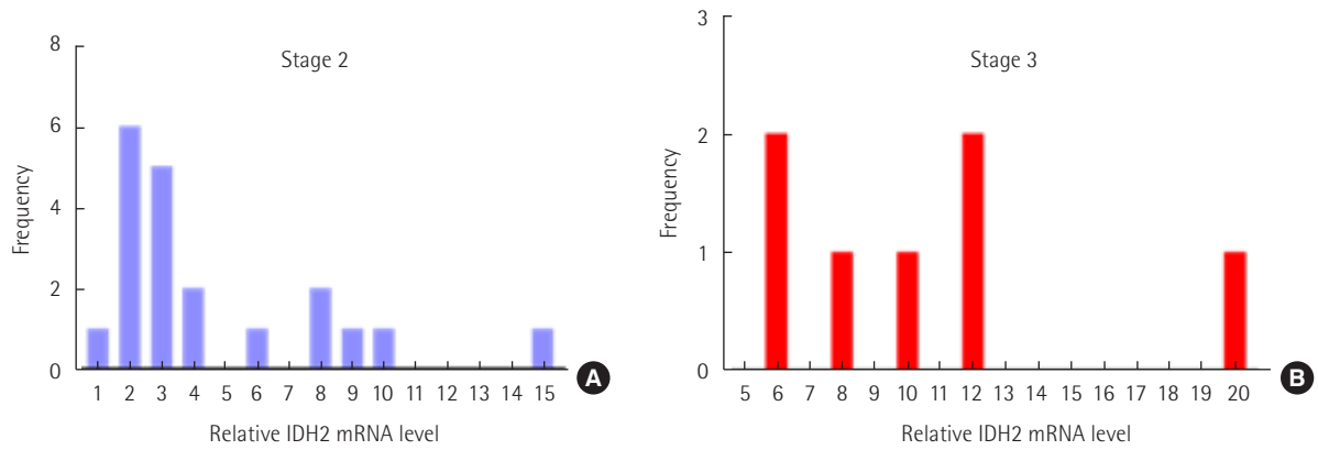
Supplementary Fig. 1. Bar graph showing the frequency distribution of the relative IDH2 mRNA level in stage 2 (A) and stage 3 (B) of human breast cancer tissues. IDH2, isocitrate dehydrogenase 2; mRNA, messenger RNA.
